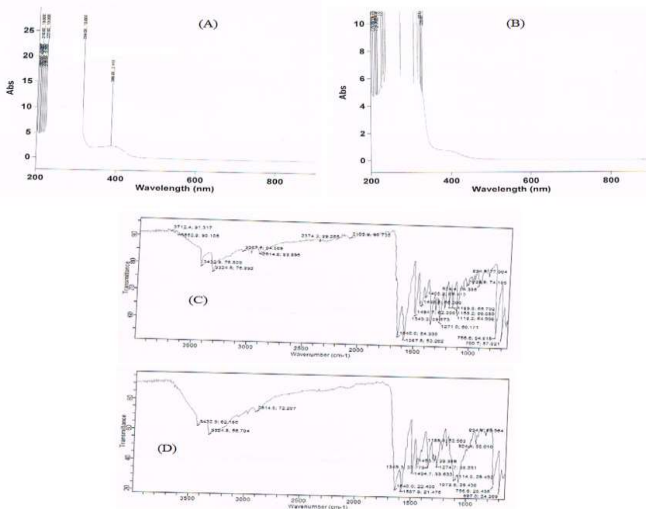
Fig. 1: UV-Vis and IR spectra of 1,5-dimethyl-2-phenyl-4-(pyrrolidin-2-ylideneamino)-pyrazolidin-3-one and complex A and C (Ligand) and B and D (Complex)
