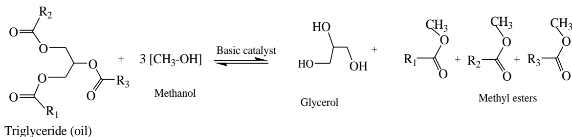
Fig. 1: Base catalyzed transesterification processes.
