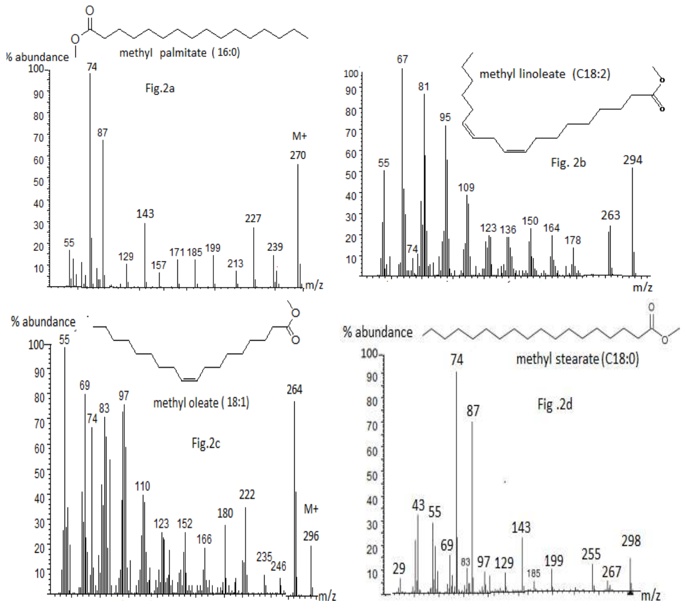
Fig. 4: Mass spectra of methyl palmitate, methyl linoleate, methyl oleate and Methyl stearate
