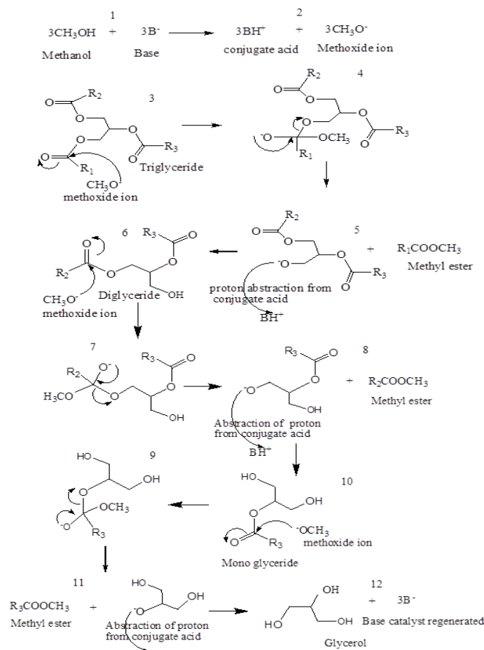
Fig. 2: Reaction mechanism for base catalyzed transesterification
