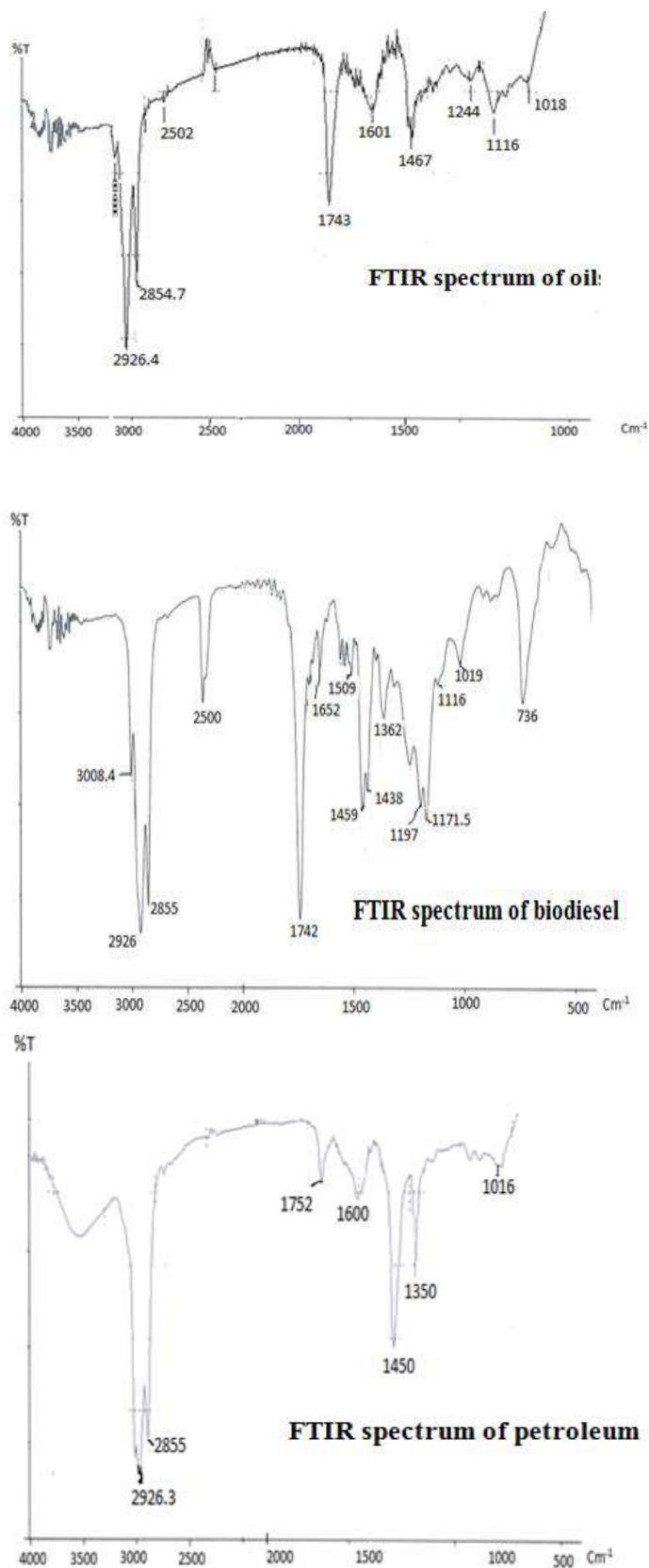
Fig. 3: FTIR spectra of oil, biodiesel and petroleum diesel
